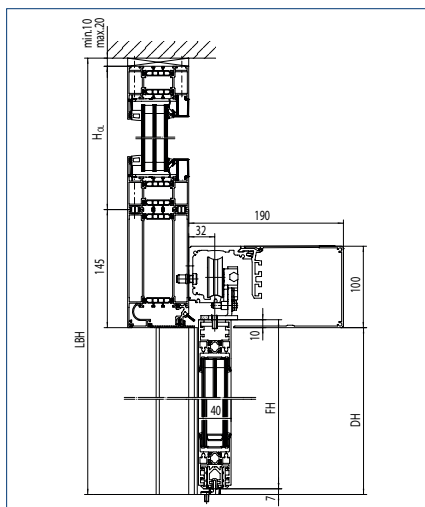
Vertical section moving leaf
