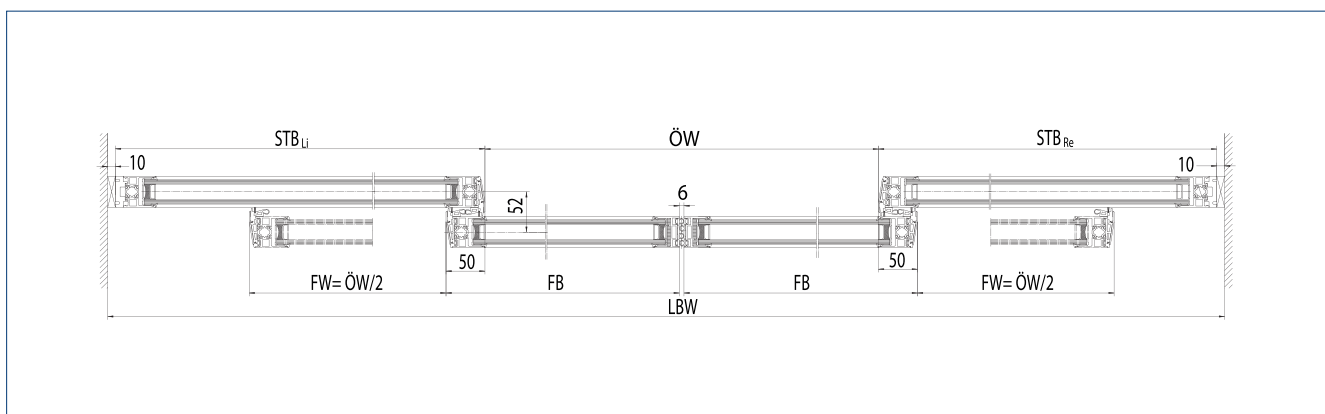
Horizontal section
